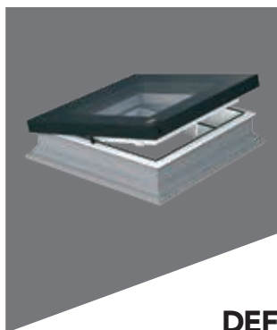
DEF SOLAR
